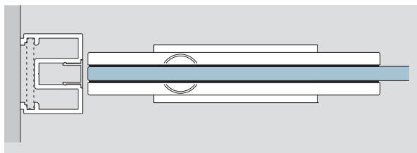
DORMA Universal Eckbeschlag, Grundriss plan DORMA Universal patch fitting
