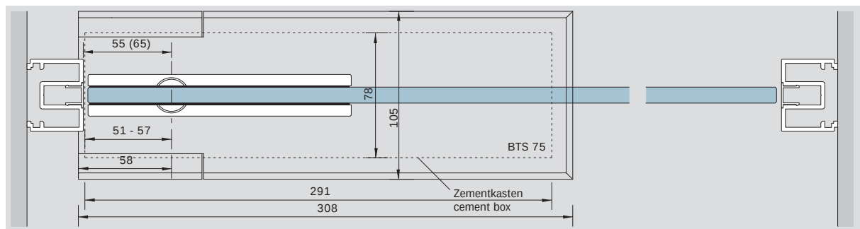
Grundriss, Pendeltür mit DORMA BTS 75 V / plan, double acting door with DORMA BTS 75 V
