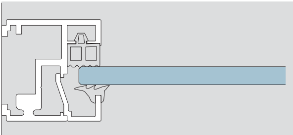
ALEXA AT 44 - Festverglasung ALEXA AT 44 - fixed glass
