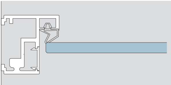
ALEXA AT 44 - Zargenprofil ALEXA AT 44 - frame profile
